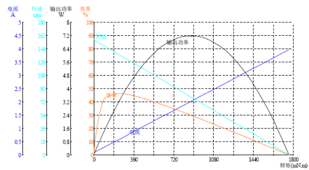
Model: WL-33RS35400128000-50K
