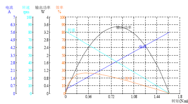
Model: WL-33RS35400067500-90K
